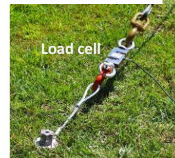
Proof Tester
